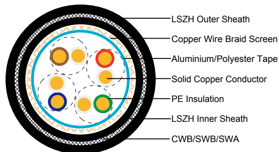
SF/UTP CAT6
