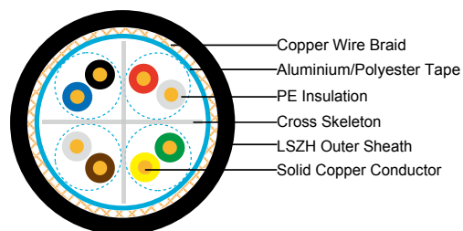
SF/UTP CAT6
